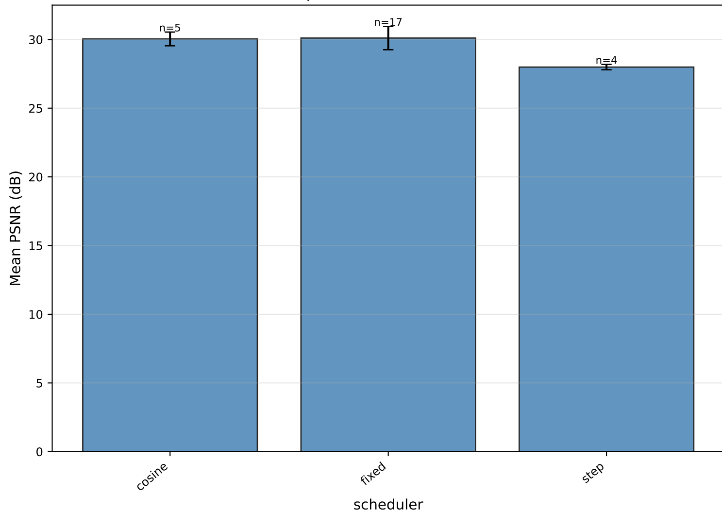
Mean PSNR per value of scheduler — SwinT
